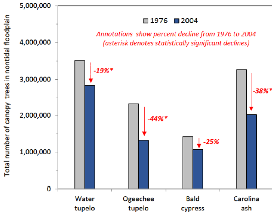
Figure 22 – Graph showing the significant decline in swamp tree species from 1976 to 2004. There were 4.3 million fewer canopy trees in 2004 than 1976 in the nontidal floodplain, 3.3 million of which were the four species in this graph. The reduction in tupelo trees is especially concerning because they are the principal source of the prized tupelo honey. Note that this figure is taken from a 2008 USGS report; more recent sampling is not available. However, continuous decreases in flow over the last decade (especially the significant and extended low-flow periods in 2007-2008 and 2011-2012) have most likely continued to harm the floodplain forest, which consists of trees that have lived for decades if not over a hundred years. This is a true and accurate copy of a chart created under my supervision, using scientifically valid methodology, that I used in my expert report (FX-790, Fig. 27). It graphically reflects data contained in an officially published USGS report, Light et al. 2008 (Table 10 and accompanying text) (FX-870).
