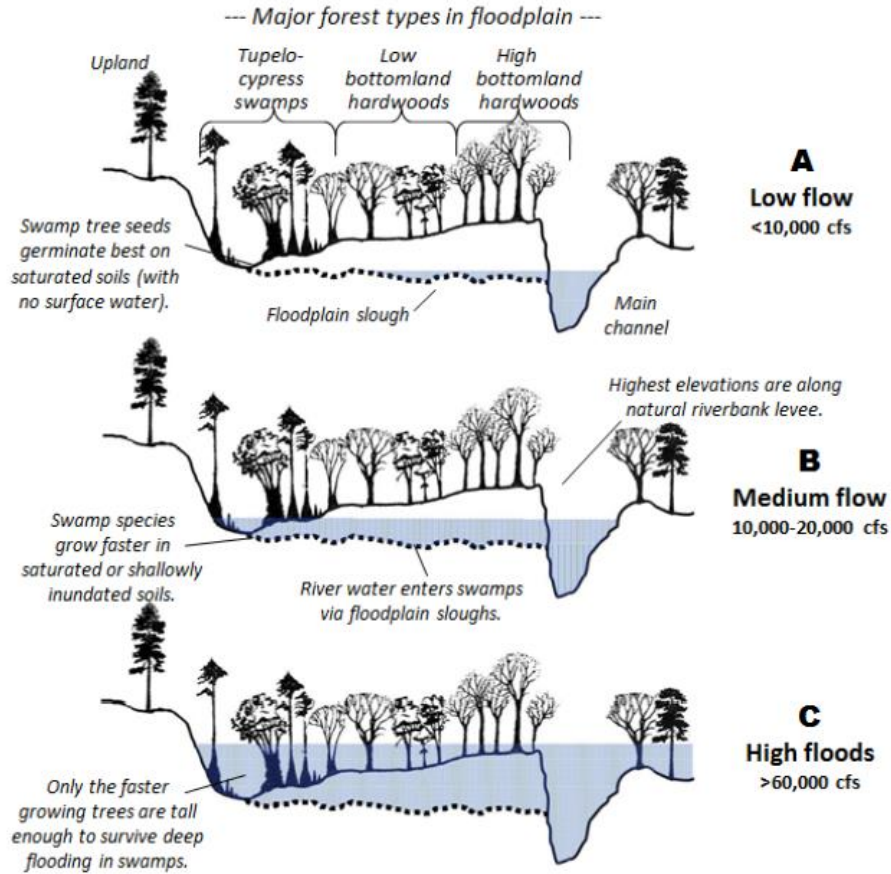
Figure 14 – This figure shows how variation in floodplain elevations and water level at which the River connects to sloughs affects the three major forest types of the Apalachicola River floodplain (tupelo-cypress swamps, low bottomland hardwoods, and high bottomland hardwoods). The caption to Figure 10 explains these types in more detail. This is a true and accurate copy of a chart that I used in my expert report (FX-790, Fig. 23). It was modified under my supervision, using generally scientifically accepted principles and methodology, from a figure published in an officially published USGS report, Light et al. 2006 (Fig. 3) (GX-88).
